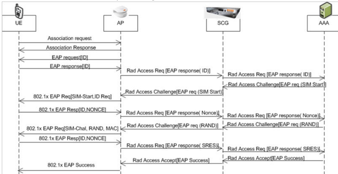
FIGURE 2 3GPP based solution sequence diagram
